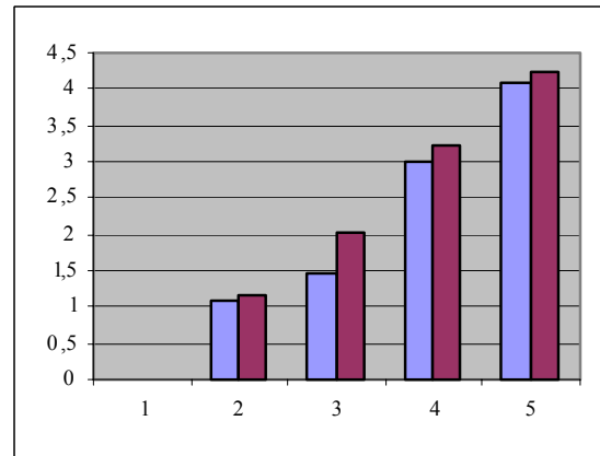
Fig. 10 Time, min., to reach curing stage 2, 20% of maximum; 3 50%; 4 80% and 5 90% of maximum for A and B at 180° C
