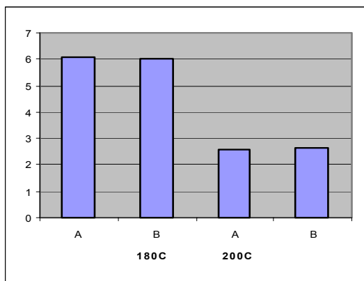
Fig. 9 Max. torque Nm at 180° C by Göttfert Rheometer and at 200° C by Monsanto MDR.
